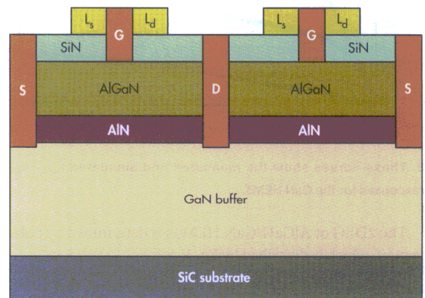
1. Depicted is the cross-sectional structure of the HEMT.
