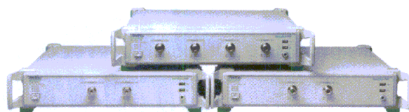
1. Low-cost ShockLine VNAs include the two-port MS46522A, four-port MS46524A, and two-port, high-frequency MS46322A for two-port testing as wide as 1 MHz to 40 GHz.
