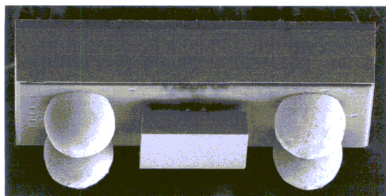
The combination of chip-scale packaging (CSP) and silicon MEMS technology make these TCXOs extremely small, boasting very low power consumption for an output frequency of 32.768 kHz for timing applications.
