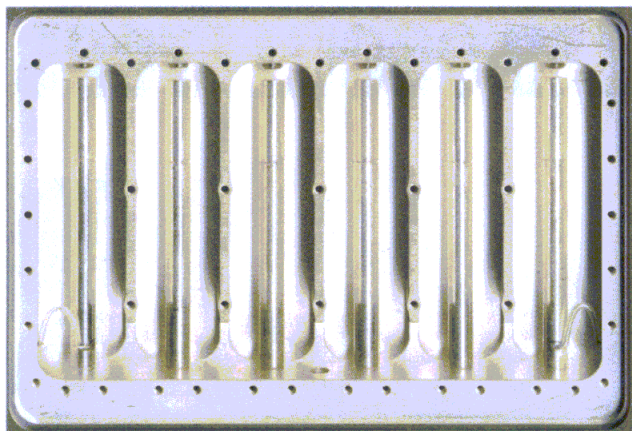
2. To enable highly precise performance, the screw elements at the end of the metallic rods in the cavity-resonator filters are adjusted outside of the housing.
