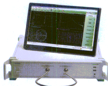
4. The ShockLine MS46322A Series VNAs provide simplified test-port-power adjustments as high as 40 GHz.
