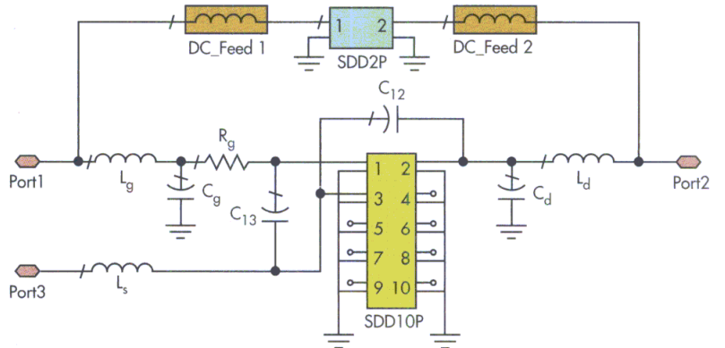
5. This block diagram shows an SDD large-signal model for the W-band HEMT.
